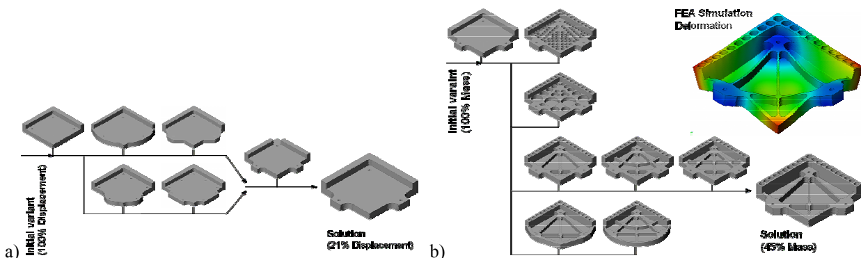
Figure 10: FEA on the measuring mirror of a NPM machine a) positioning of the supporting points and reducing the deflection and b) reducing of the mirror mass
